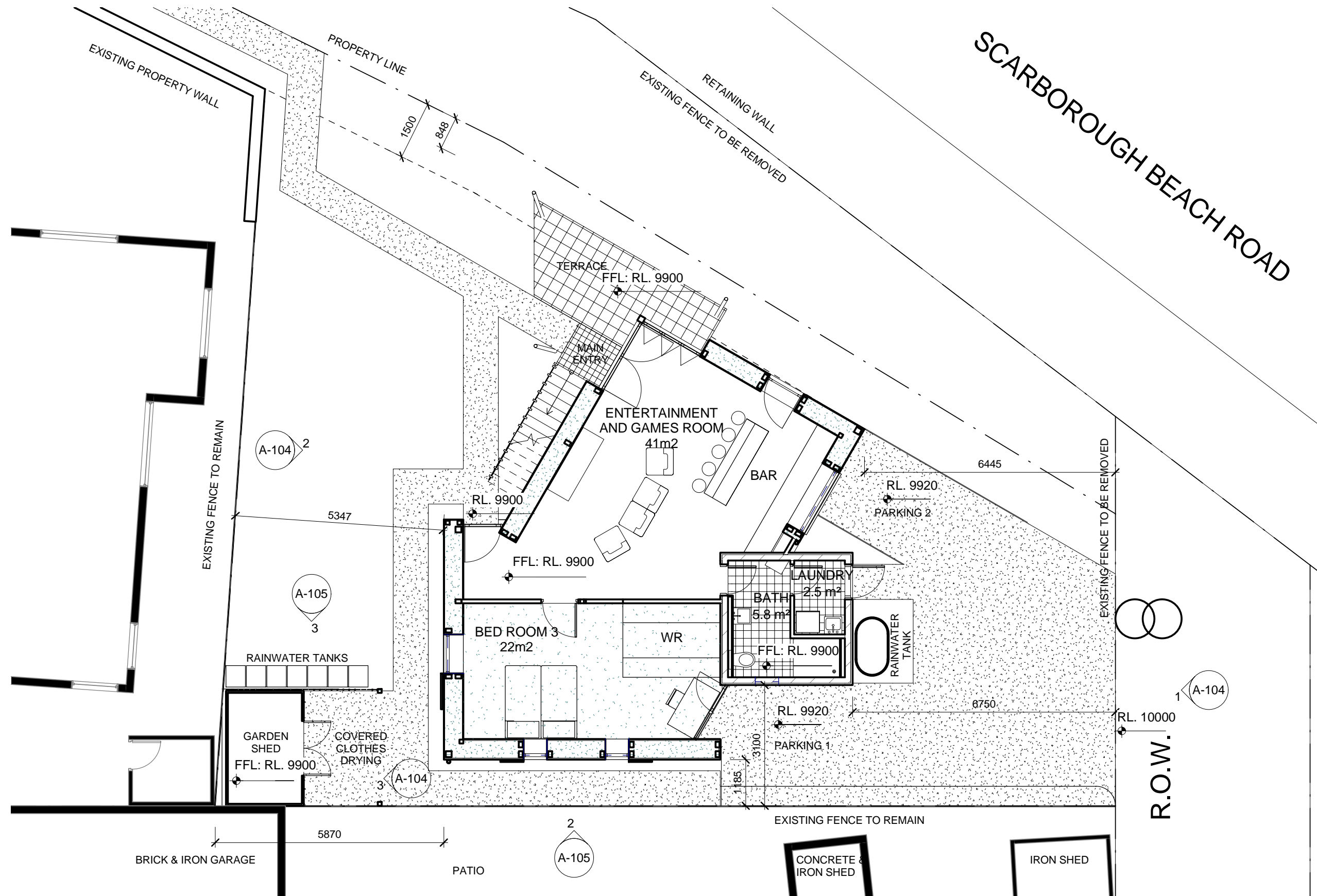
1 Ground Floor Plan A-104 1 : 100
