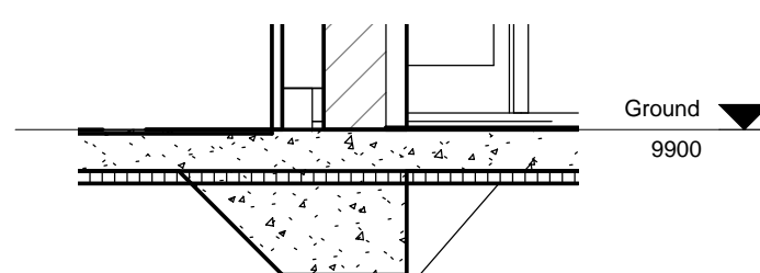
2 Detail Section Bath West A-301 1:20
