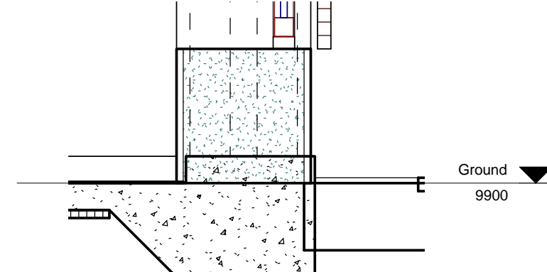
3 Detail Section West Wall A-301 1:20
