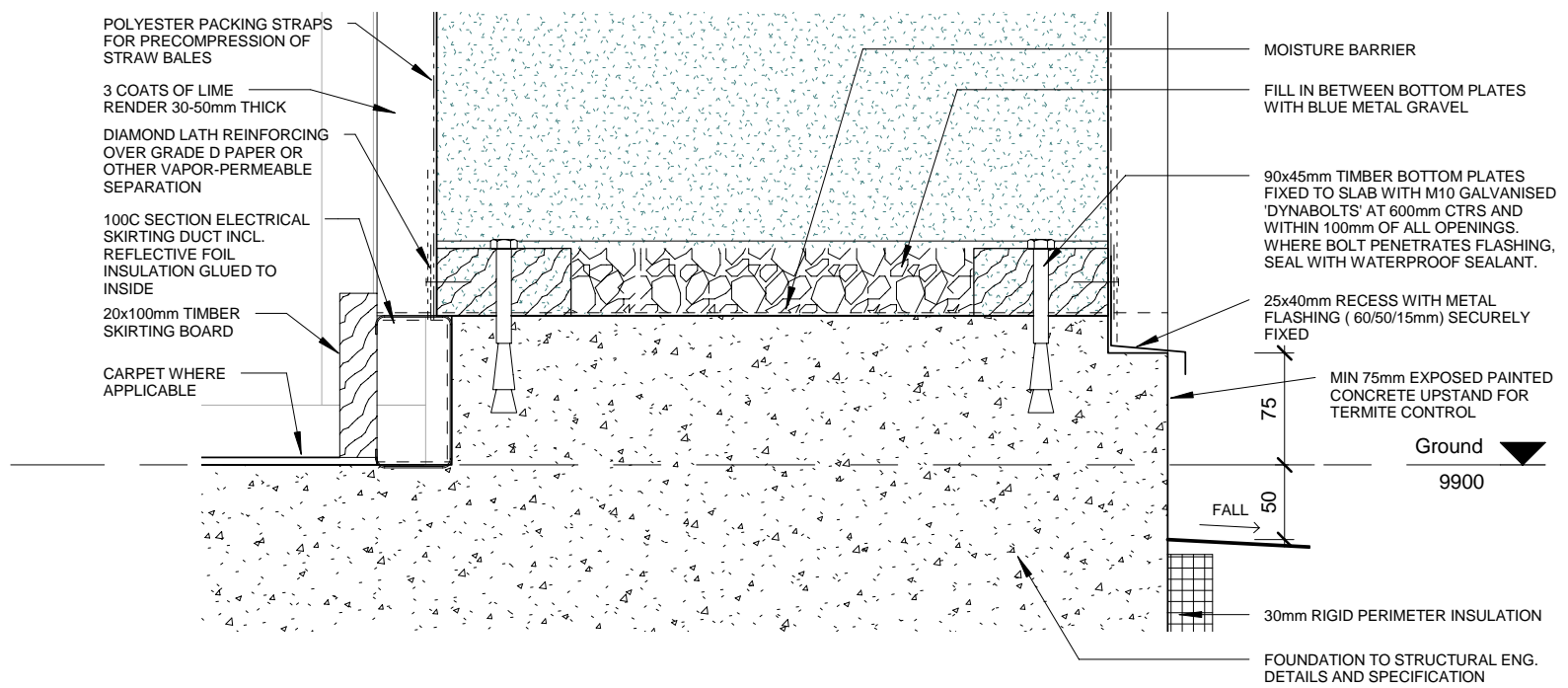
1 Typical Detail - Footing Wall Connection A-350 1:5
